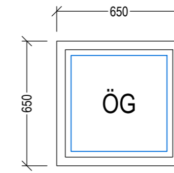
GL-01 - 3 Stk Mkv = 1:20
