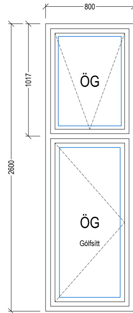
GL-08 - 1 Stk Mkv = 1:20
