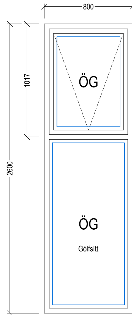
GL-05 - 7 Stk Mkv = 1:20
