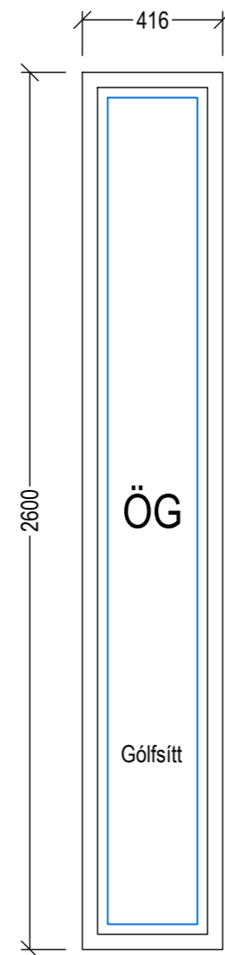
GL-06 - 1 Stk Mkv = 1:20
