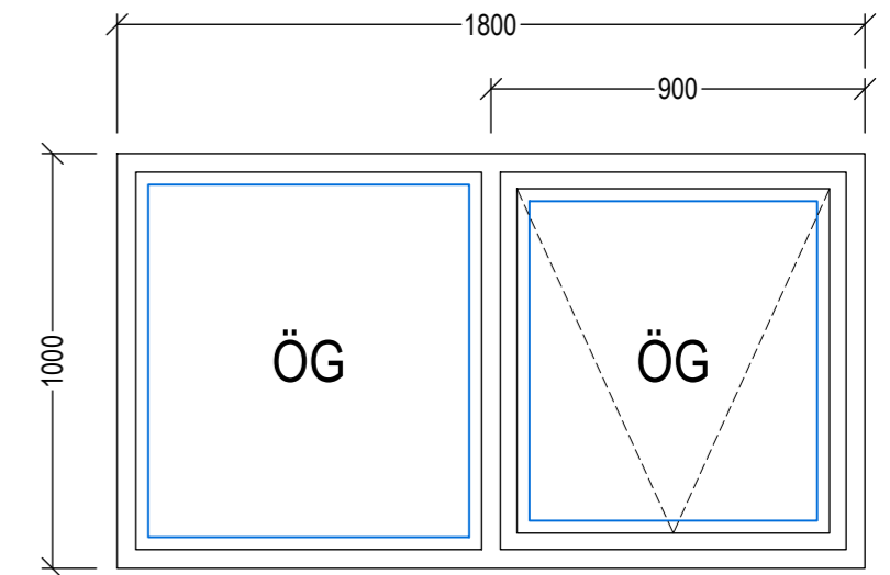
GL-03 - 7 Stk Mkv = 1:20
